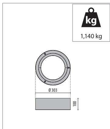
311009 - COVER
