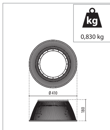
311019 - POLYCARBONATE DIFFUSER
