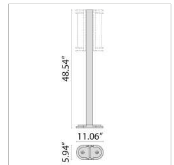
P48 48.54" Post
