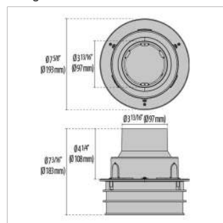
Rough-in Kit CRICKET+ 10 RGBW/TW
