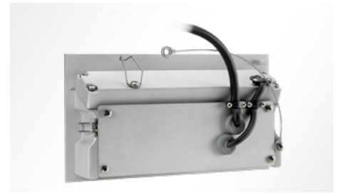
Pre-wired cable is factory sealed to housing with a cable gland allowing external electrical connections.
