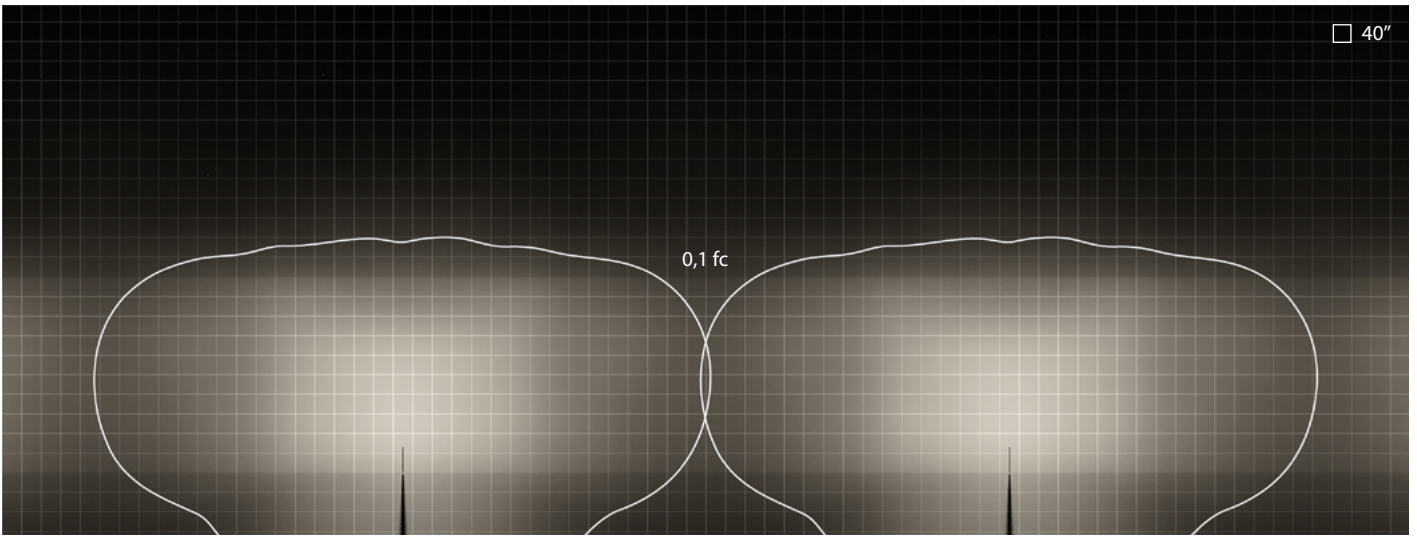
SYSTEMLINE+ | IESNA Type distribution | TYPE II | linear
