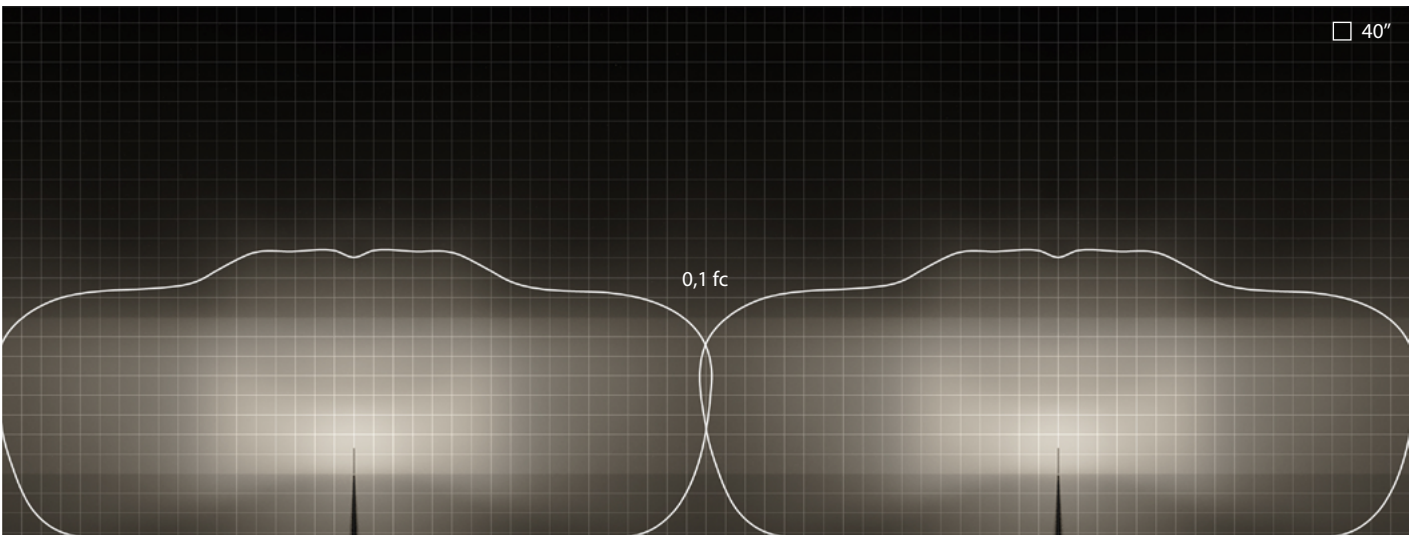
SYSTEMLINE+ | IESNA Type distribution | TYPE I | linear
