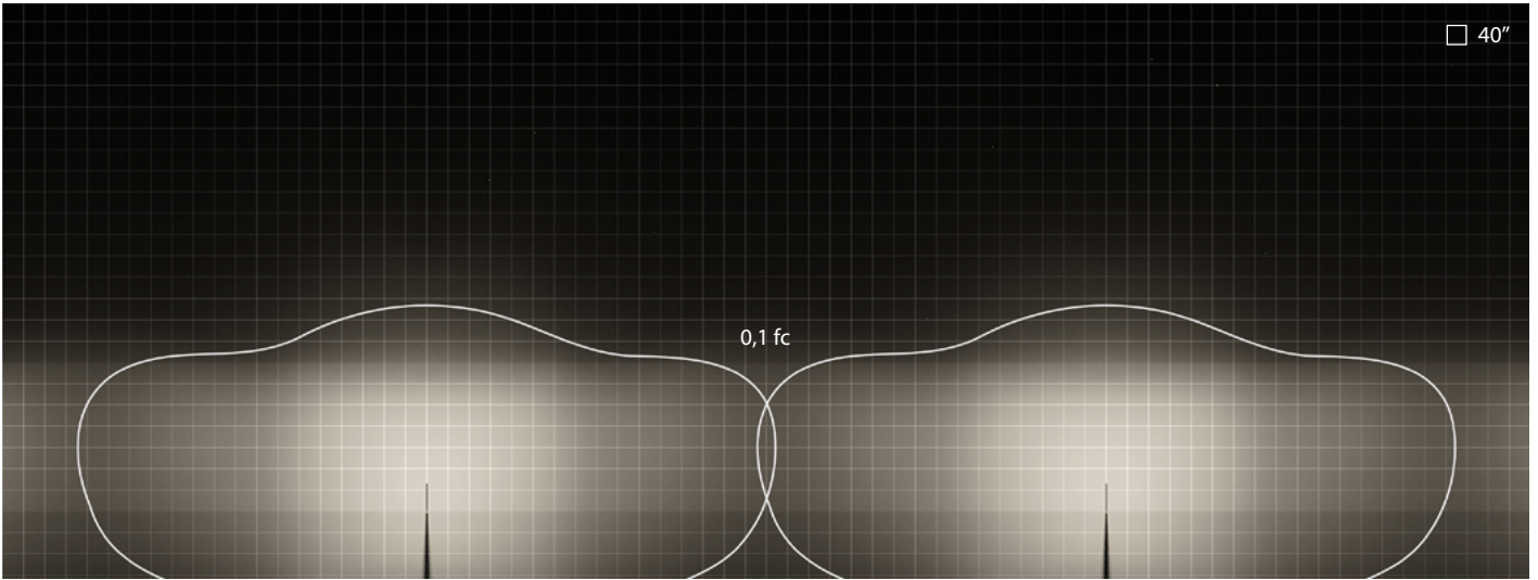
SYSTEMLINE+ | A/W Asymmetric Wide optics | TYPE II | linear
