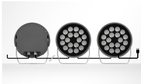
Each luminaire is supplied with two IP 68 cable glands allowing a single or a through power connection
